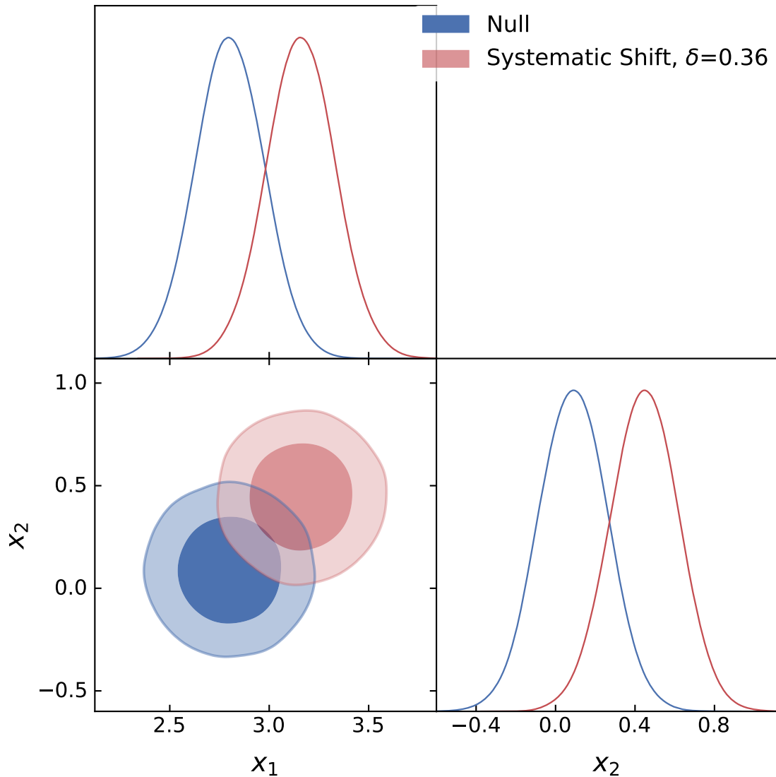
Data realisations: Null vs. Systematic Shift \delta
